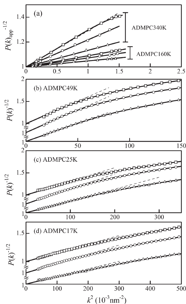
Figure 1. Angular dependence of P(k)_{app}^{-1/2} (from SLS) or P(k)^{-1/2} (from SAXS) for indicated ADMPC samples in MIBK (squares), MEK (circles), and MEA (triangles) at 25 °C.
