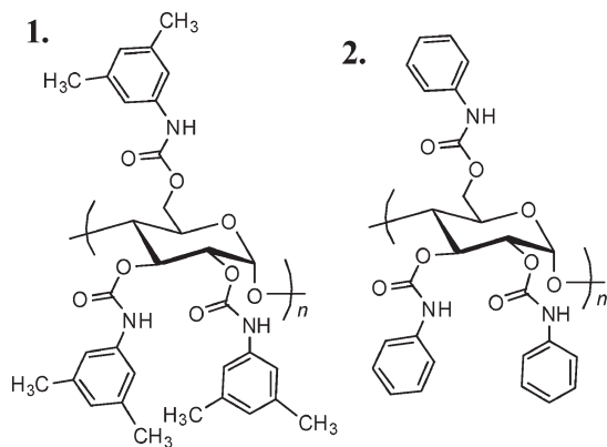
Chart 1. Chemical Structures of ADMPC (1) and ATPC (2)
