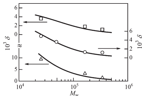
Figure 4. Molecular weight dependence of the optical anisotropy factor \delta for ADMPC in MIBK (squares), MEK (circles), and MEA (triangles) at 25 °C. The curve represents the theoretical values calculated from eq 9 (see text for the parameters).
